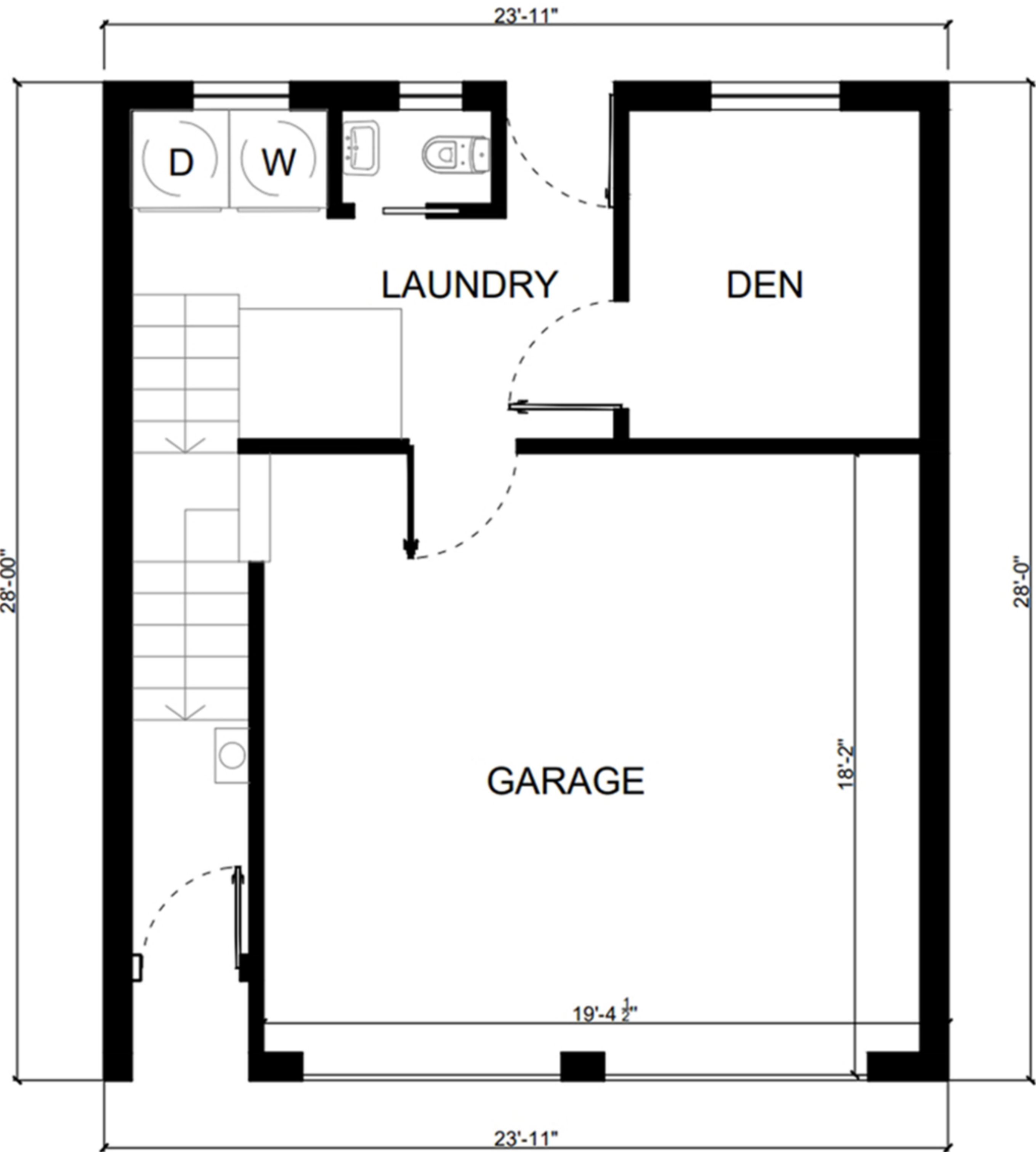
PROPOSED LOWER FLOOR
