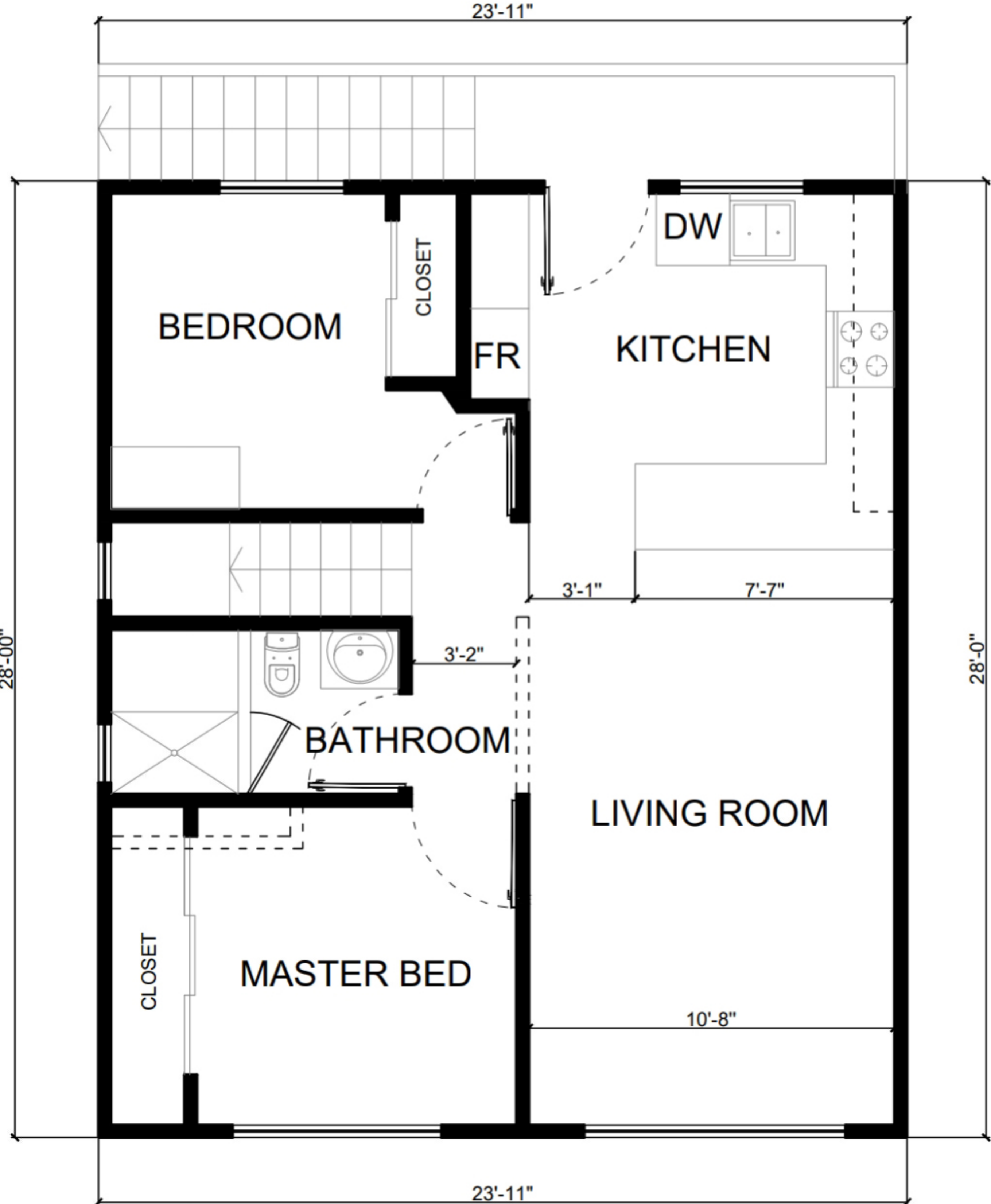
PROPOSED UPPER FLOOR
